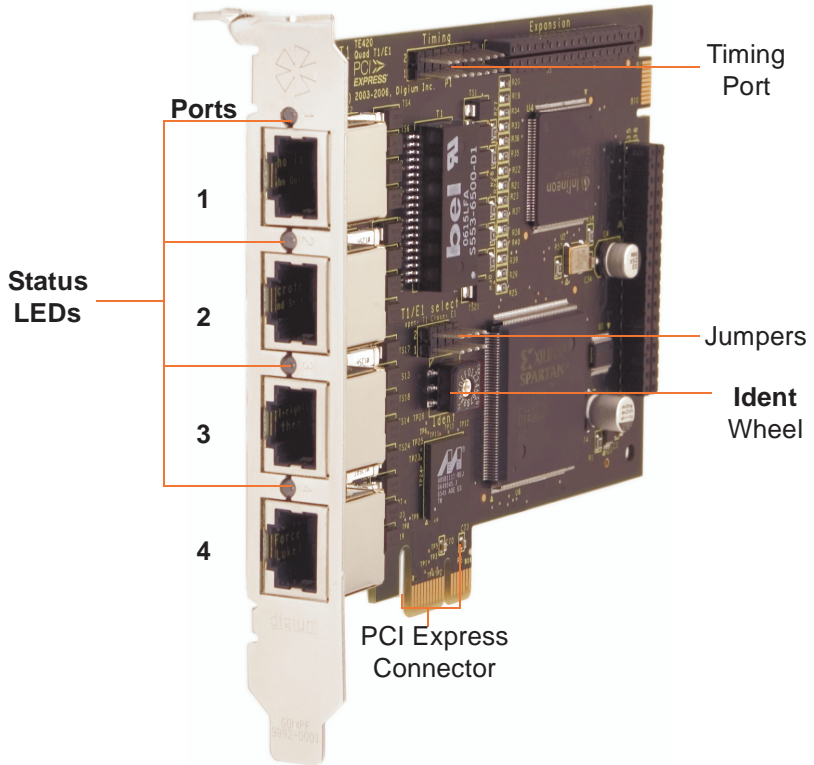
Figure 5: TE420 Card
